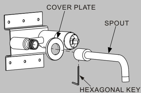
FIG. 1 INSTALLATION OF SPOUT
