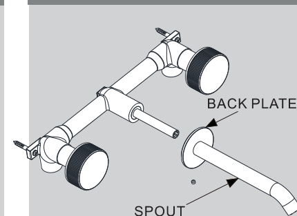
FIG. 3 INSTALLATION OF SPOUT
