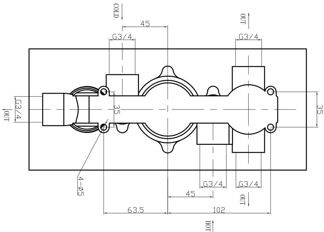
DE3000RC - DESIGN THERMOSTATIC SHOWER VALVE 3 Way Diveter
