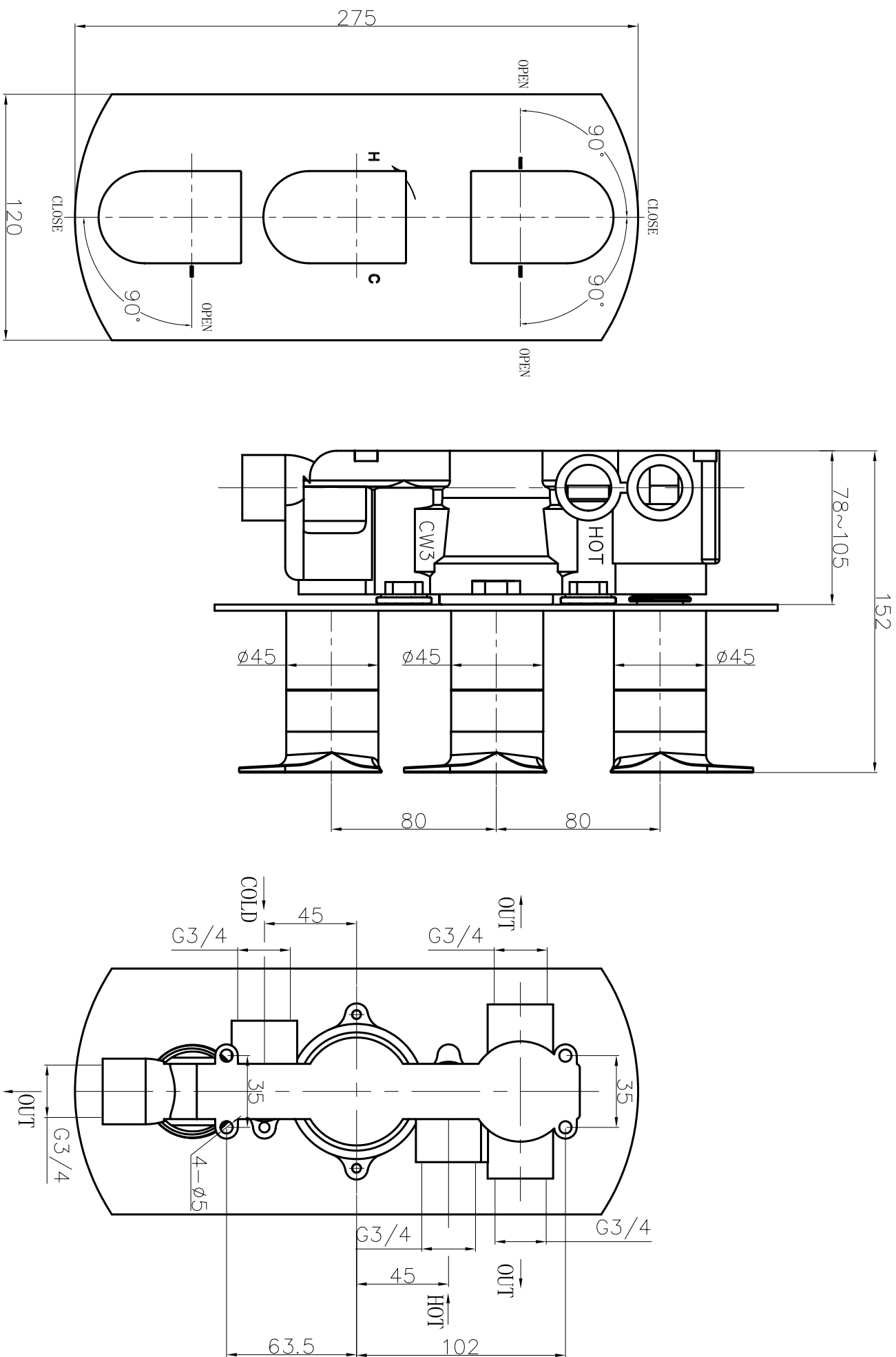
MO3000RC - MODEST THERMOSTATIC SHOWER VALVE 3 Way Portrait
