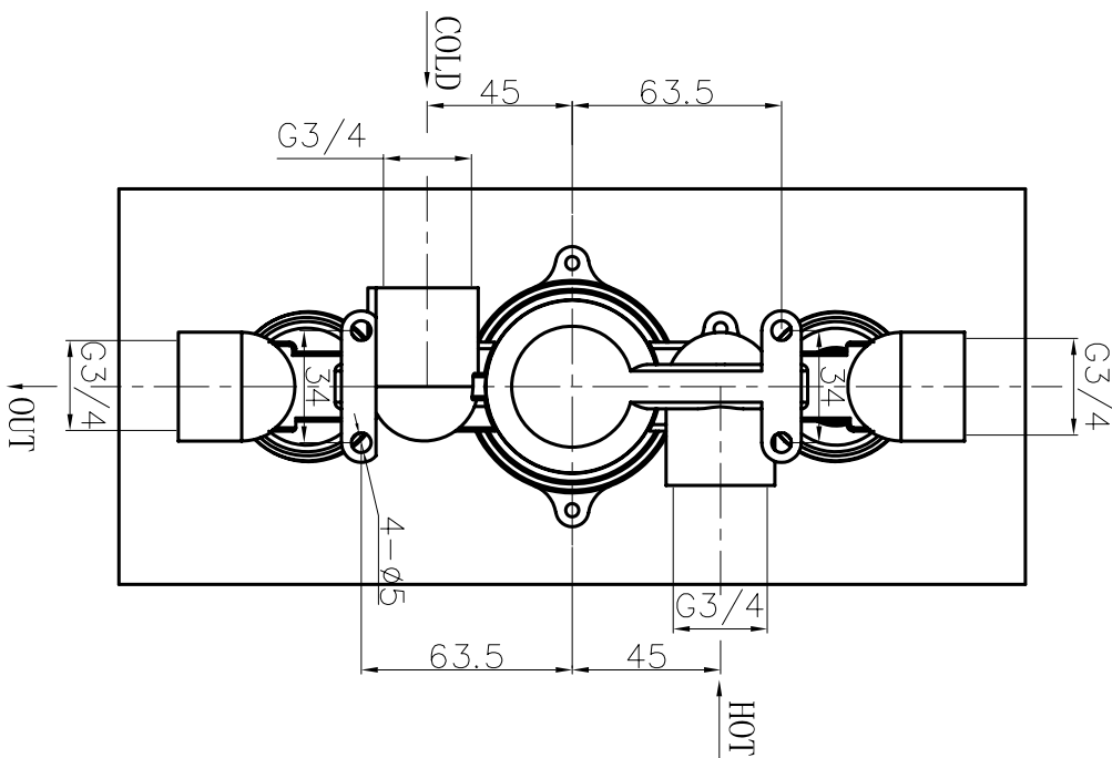
WS2000RC - WATERSQUARE THERMOSTATIC VALVE 2 Way Portrait
